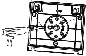
5.1.1. Drill through the mounting hole with an electric drill.
