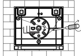
5.1.2 Lock the bottom shell on the mounting seat with screws.
